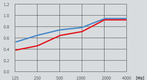
\alpha_s Schallabsorptionsgrad
