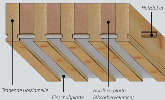
BRESTA® Akustik Gentle HF 40 Schallabsorptionsgrad \alpha_w = 0.80
